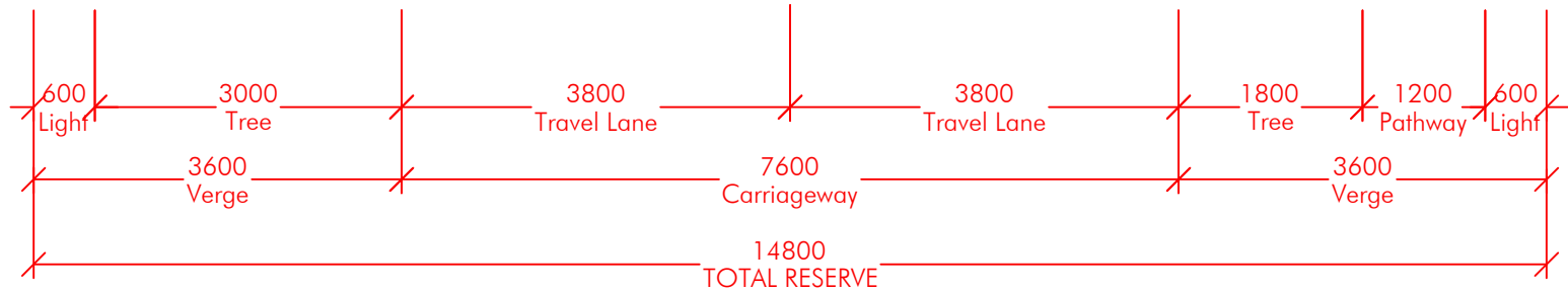
INDICATIVE 14.8m LOCAL MINOR ROAD STREETSCAPE (ROADS 602, 603, 604, 605) SCALE 1:75
