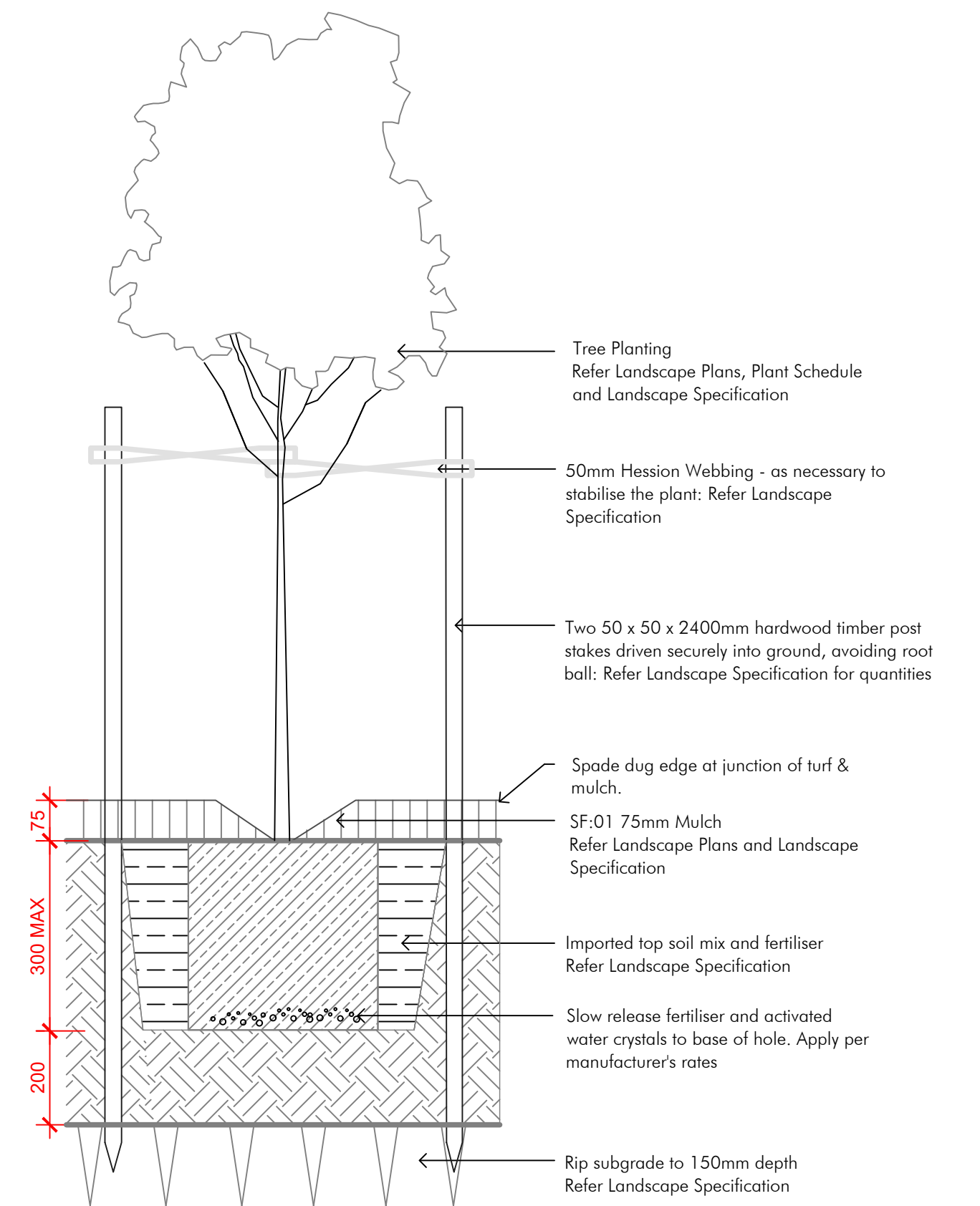
TREE PLANTING (NON STREET TREE) SCALE 1:10
