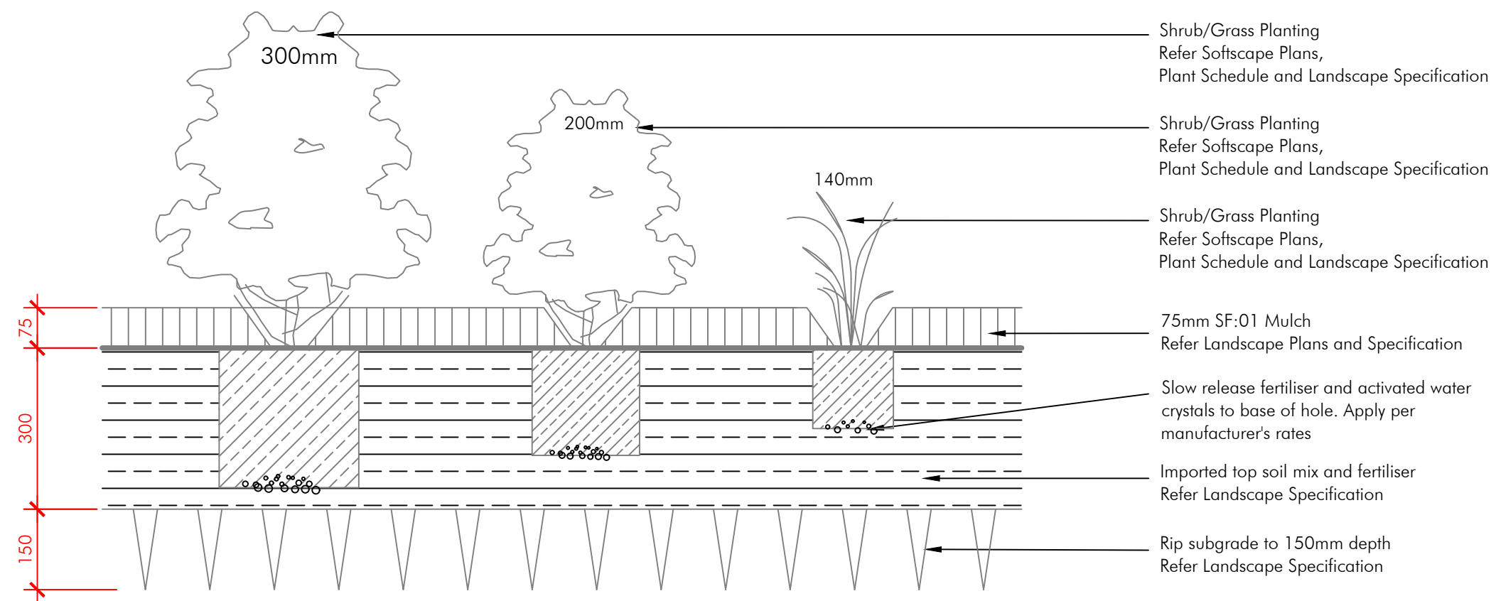
SHRUB, ACCENT & NATIVE GRASS PLANTING SCALE 1:10
