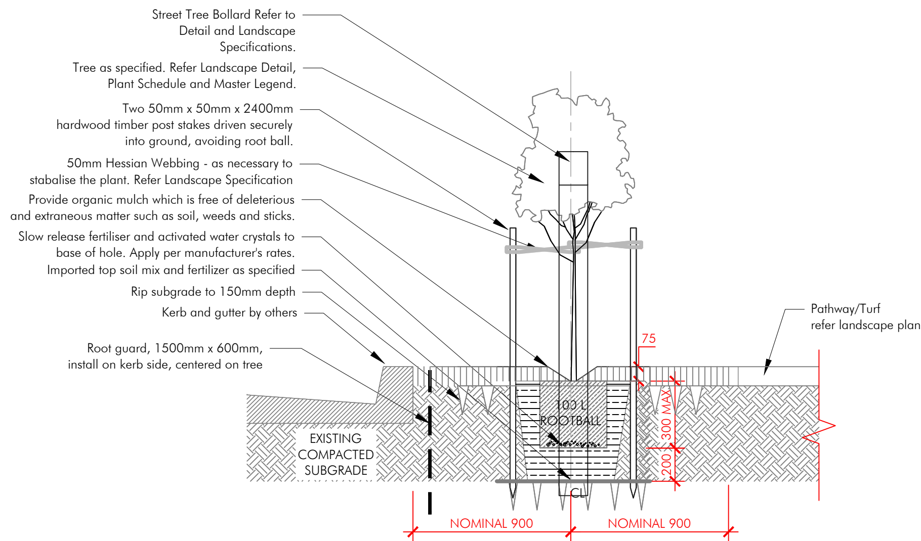
TYPICAL STREET TREE DETAIL - MINOR LOCAL ROAD SCALE 1:20
