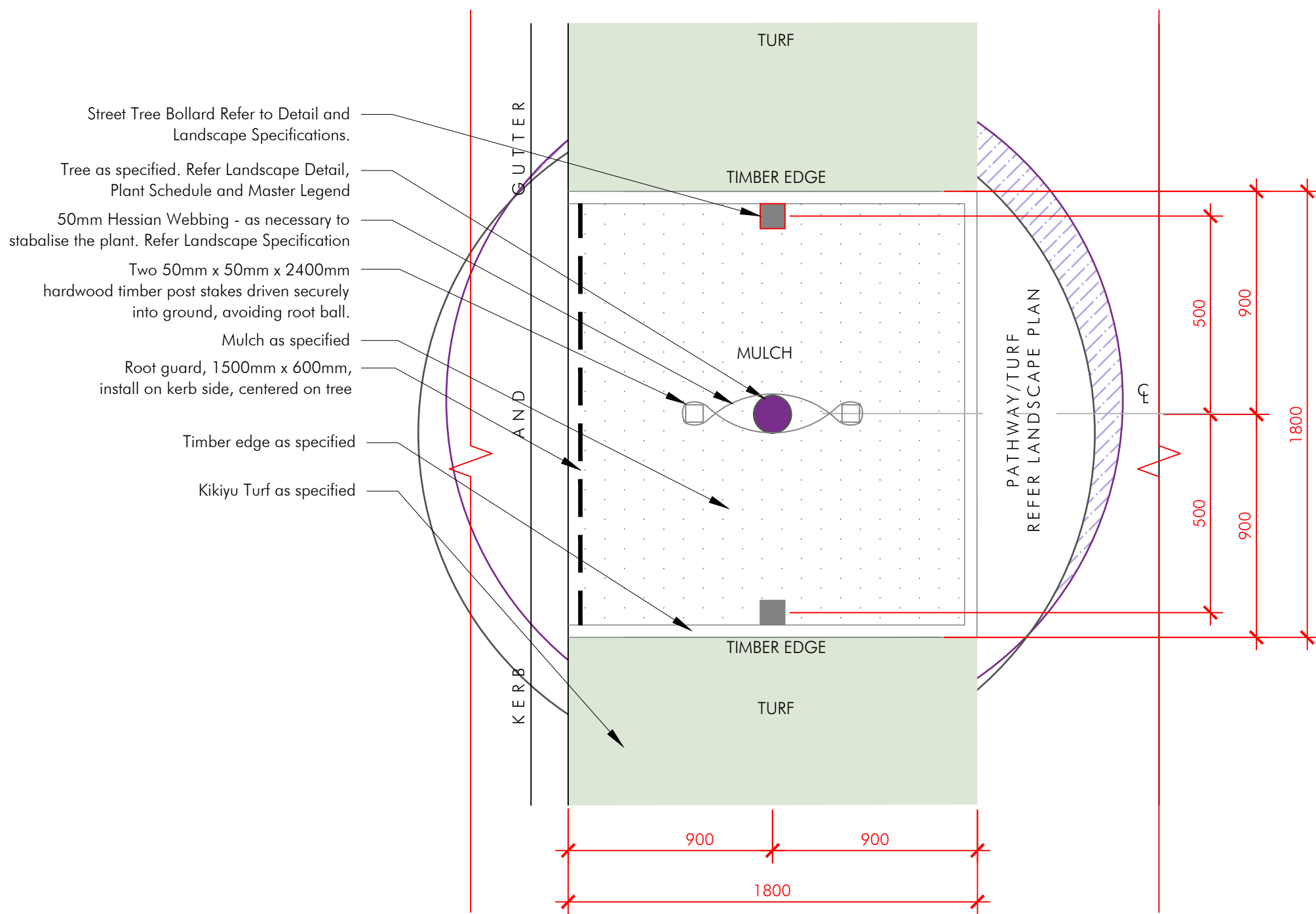
TYPICAL STREET TREE PLAN - MINOR LOCAL ROAD SCALE 1:20
