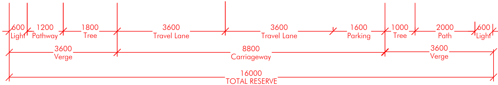
INDICATIVE 16.0m LOCAL STREETSCAPE (ROAD 601) SCALE 1:75
