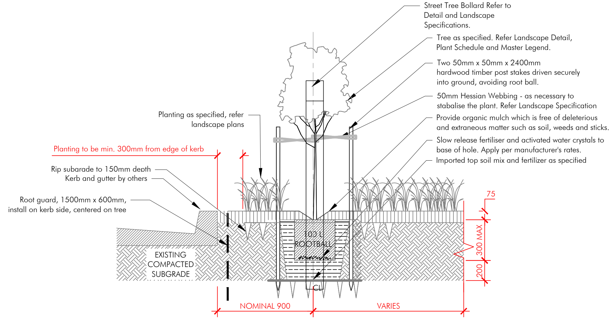
TYPICAL STREET TREE IN BLISTER DETAIL - LOCAL ROAD SCALE 1:20
